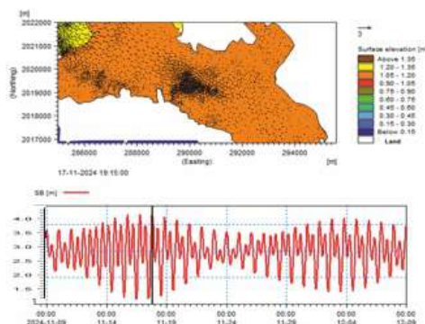
Figure 5: Results obtained for Hydrodynamic Model for Spring and neap tide (Existing)
