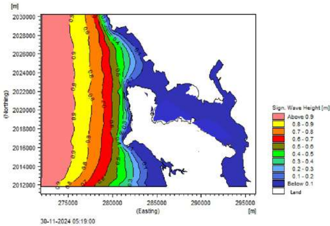
Figure 8: Spectral Wave Modelling: Existing and Proposed
