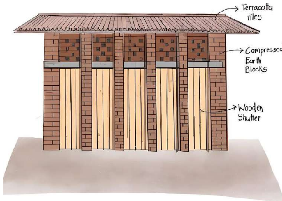
Figure 2-CSEB Composite Design (Source -Authors)
